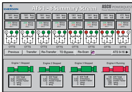
Fig. 23: ASCO POWERQUEST® 32.15
